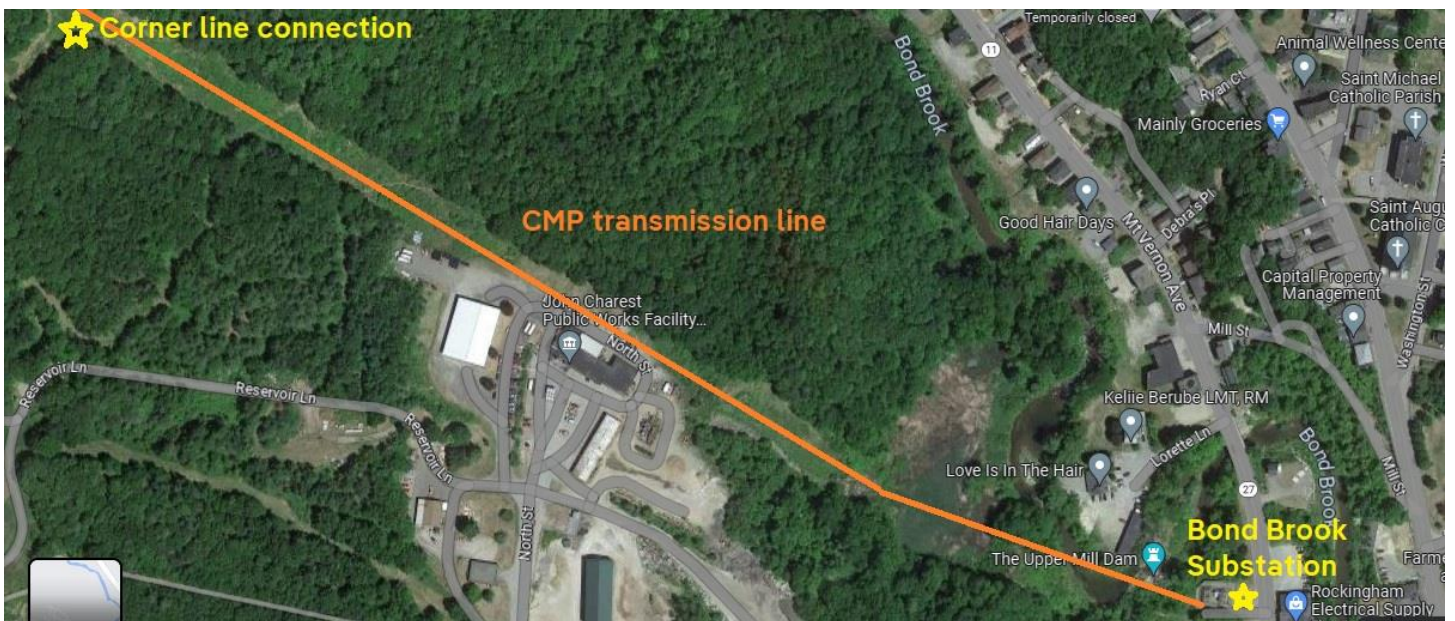
Central Maine Power will be rebuilding a transmission line that connects to another line in the Bond Brook Recreation Area and to the Bond Brook Substation on Mount Vernon Road in Augusta. The City of Augusta's Public Works building is adjacent to this line. Work will begin in the Fall or early Winter 2023.
